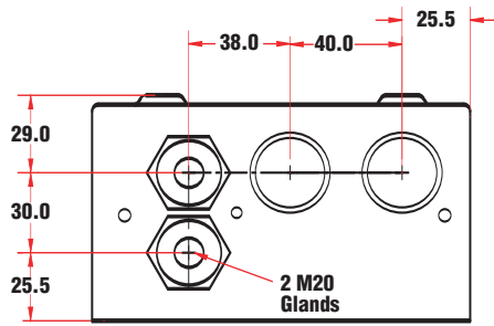
Dimensions of piped exhaust docking station
